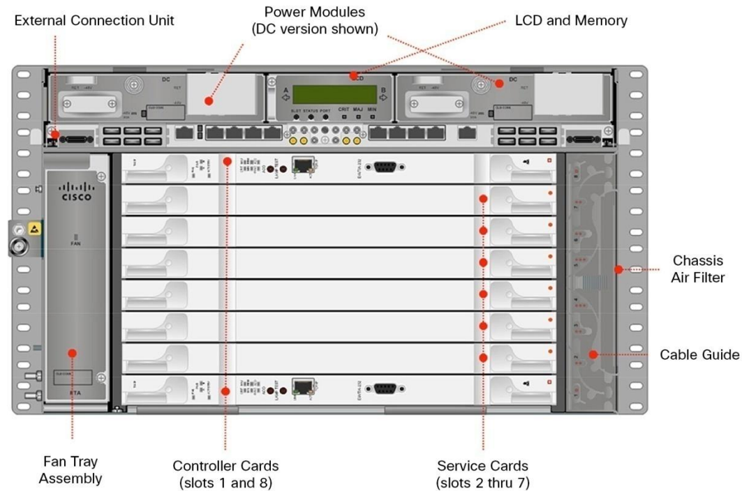
Figure 4. Cisco NCS 2006
