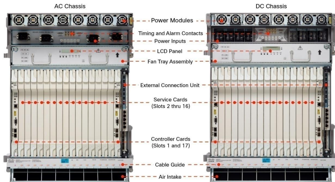
Figure 2. Cisco NCS 2015
